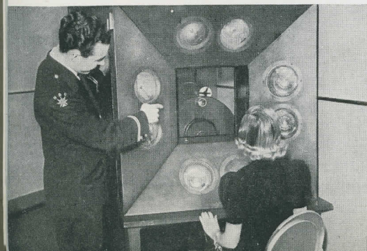
Outmoded mechanical scanning camera. Subject sat before photoelectric cells.
