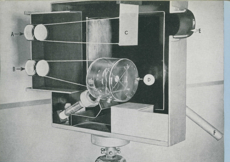
Simplified cutaway model of television studio camera, indicating principal parts. A—Focusing lens for ground-glass. B—Lens which focuses image on Iconoscope plate. C—Ground glass. D—Iconoscope. E—Viewing aperture which permits operator to see the ground-glass. F—Focusing handle.
