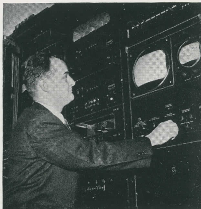
Section of transmitter control board in the Empire State Building.
