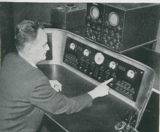
Master control board of NBC's television transmitter station, located on the 85th floor of the Empire State Building.
