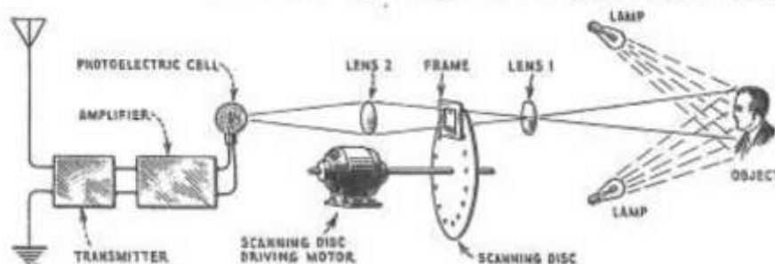
Fig. 2 - PROGRESSIVE OBSERVATION AS A SCANNING METHOD
