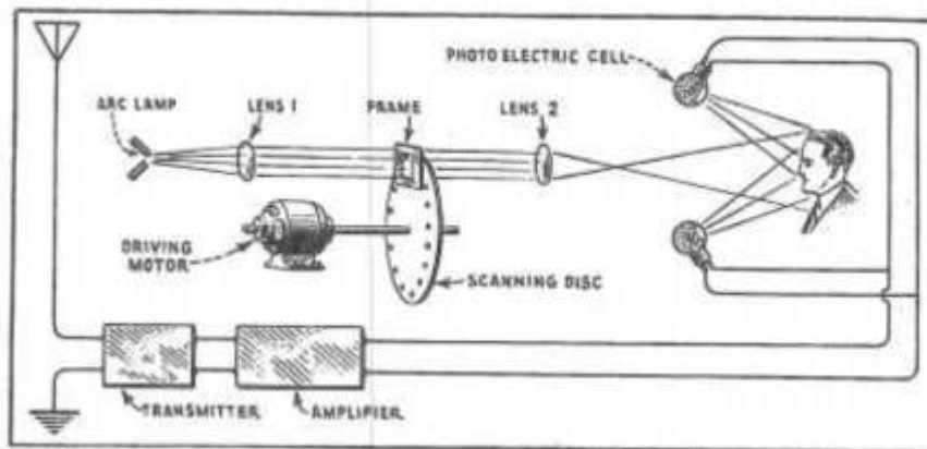
Fig. 3 - PROGRESSIVE ILLUMINATION AS A SCANNING METHOD
