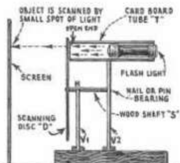
Fig. 16 - ILLUSTRATING PRINCIPLE OF SCANNING BY PROGRESSIVE ILLUMINATION
