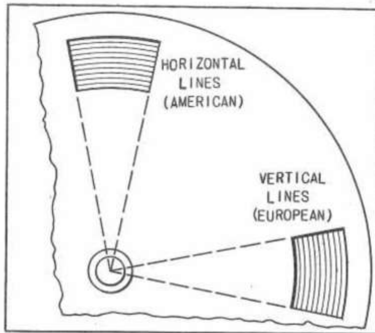
Fig. 4 - A SCANNING DISC MAY BE USED FOR EITHER HORIZONTAL OR VERTICAL SCANNING
