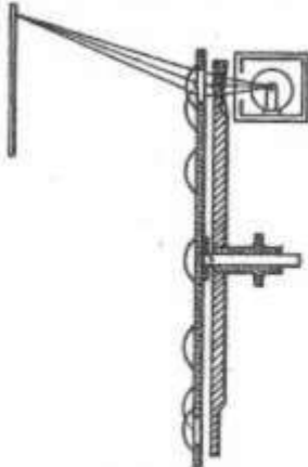
Fig. 6 - LENS AND PRISM DISCS SEPARATELY PROVIDE TWO COMPONENTS OF SCANNING MOTION
